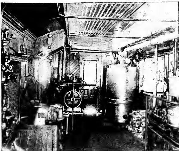
Fig. 219. INTERIOR AIR BRAKE INSTRUCTION CAR.
